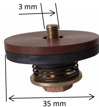
Exhaust Valve P/N:0916000696 POS:159# For Model: RA0025/0040 RA0063/0100
