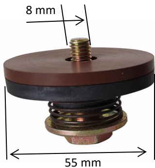
Exhaust Valve P/N:0916516777 POS:159# For Model: RA0160/0202 RA0250/0302
